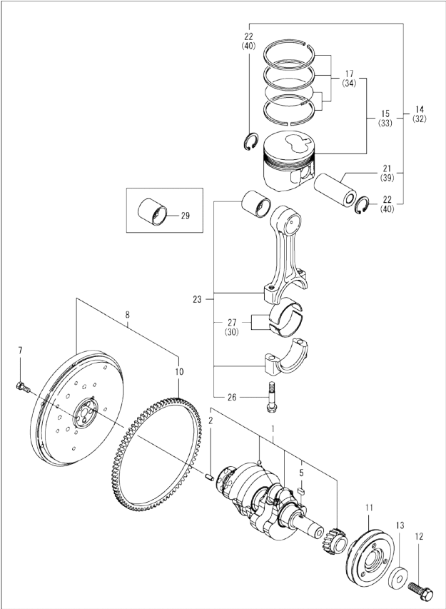
Fig.7. CRANKSHAFT & PISTON
